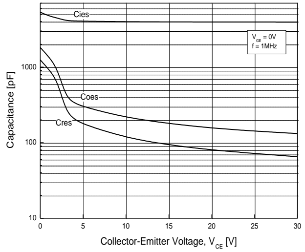
Fig.8 Typical Capacitance
